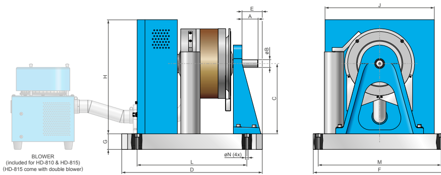
Fig. 5: HD-810 Dynamometer with short base plate and blower
