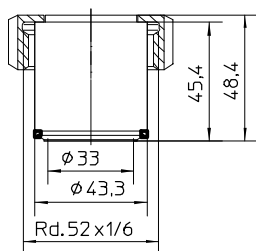
HYGENIC-Tubus * Ø 43.3 with screwing DN25/PN40
