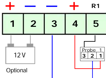
Connection of probes and eventual battery
